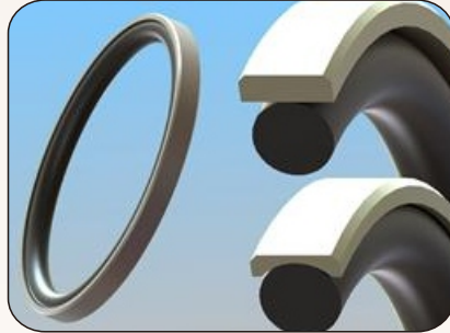
Glyd Ring
